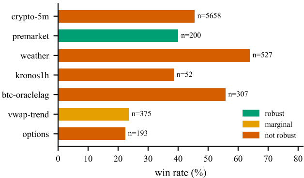
Win rate by strategy, shaded by Monte-Carlo verdict
