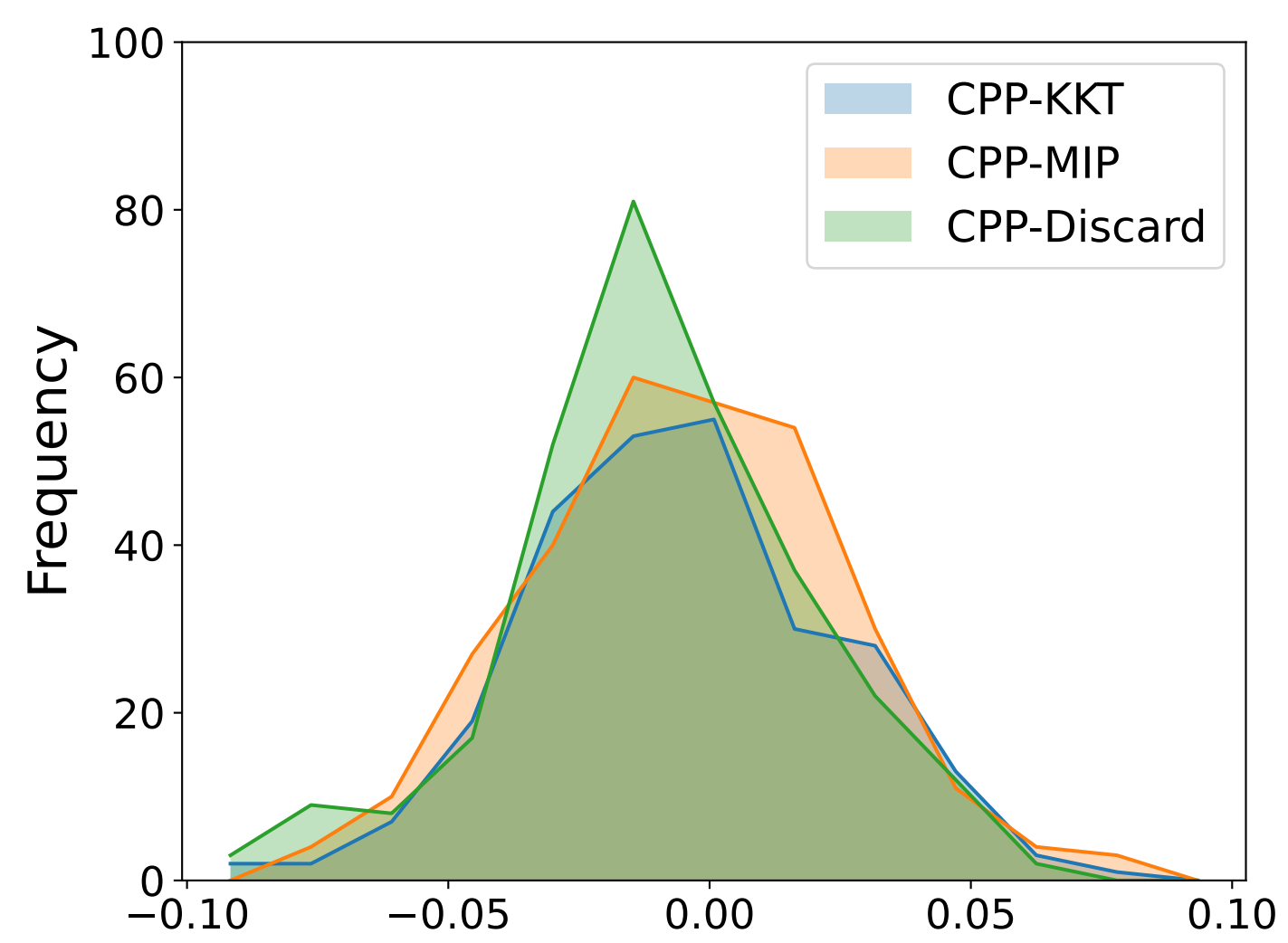
(a) C_m(x_m^*)
