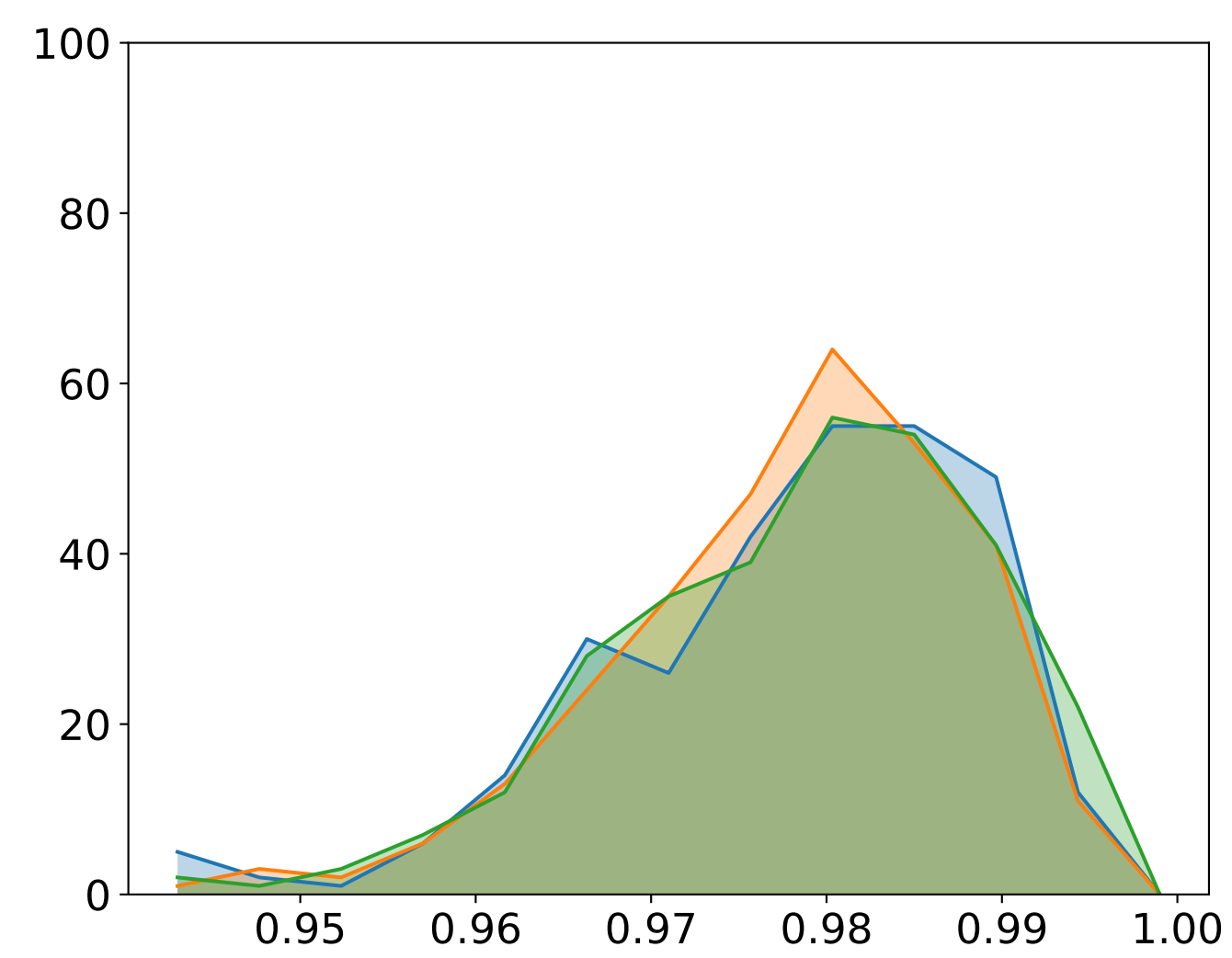
(c) CEC_{c,l}
