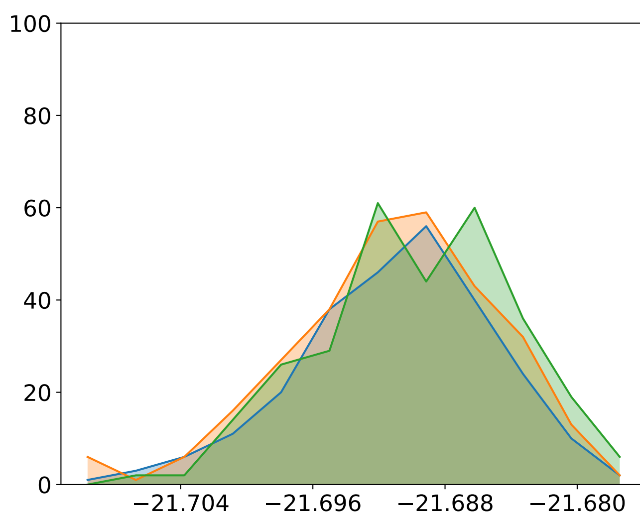
(b) J(x_m^*)
