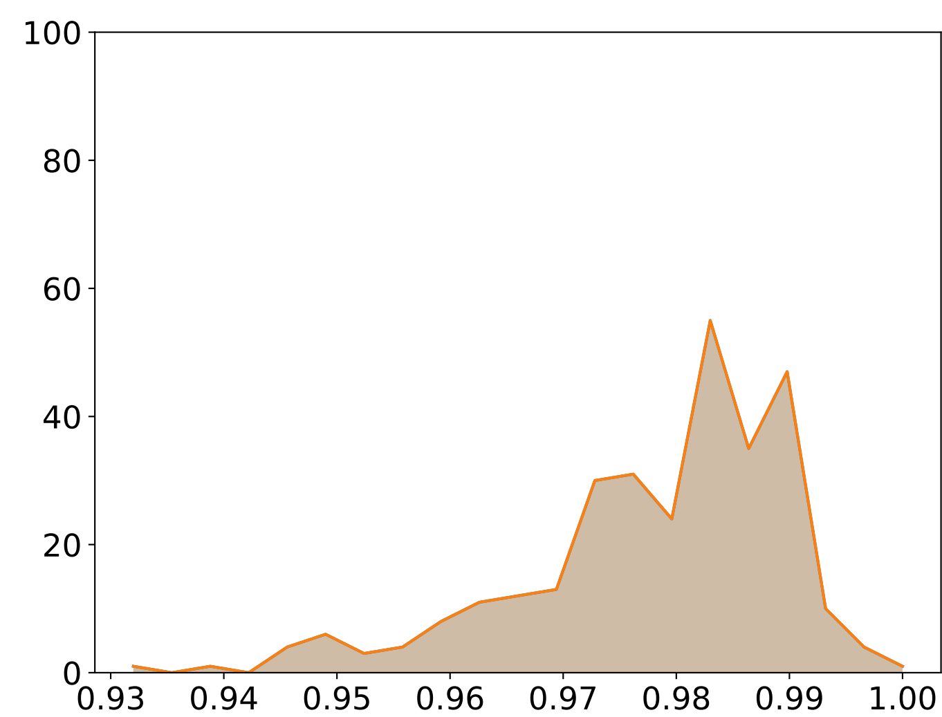
(c) CEC_{c,l}
