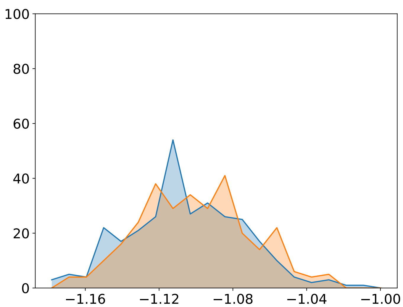
(b) J(x_m^*)
