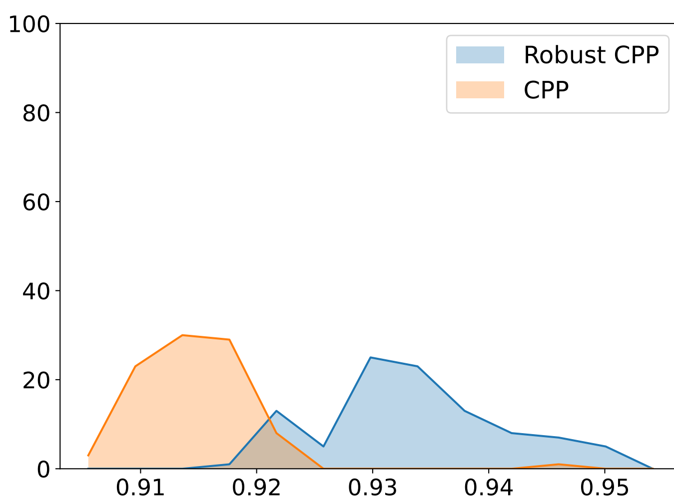
(b) J(x^*)
