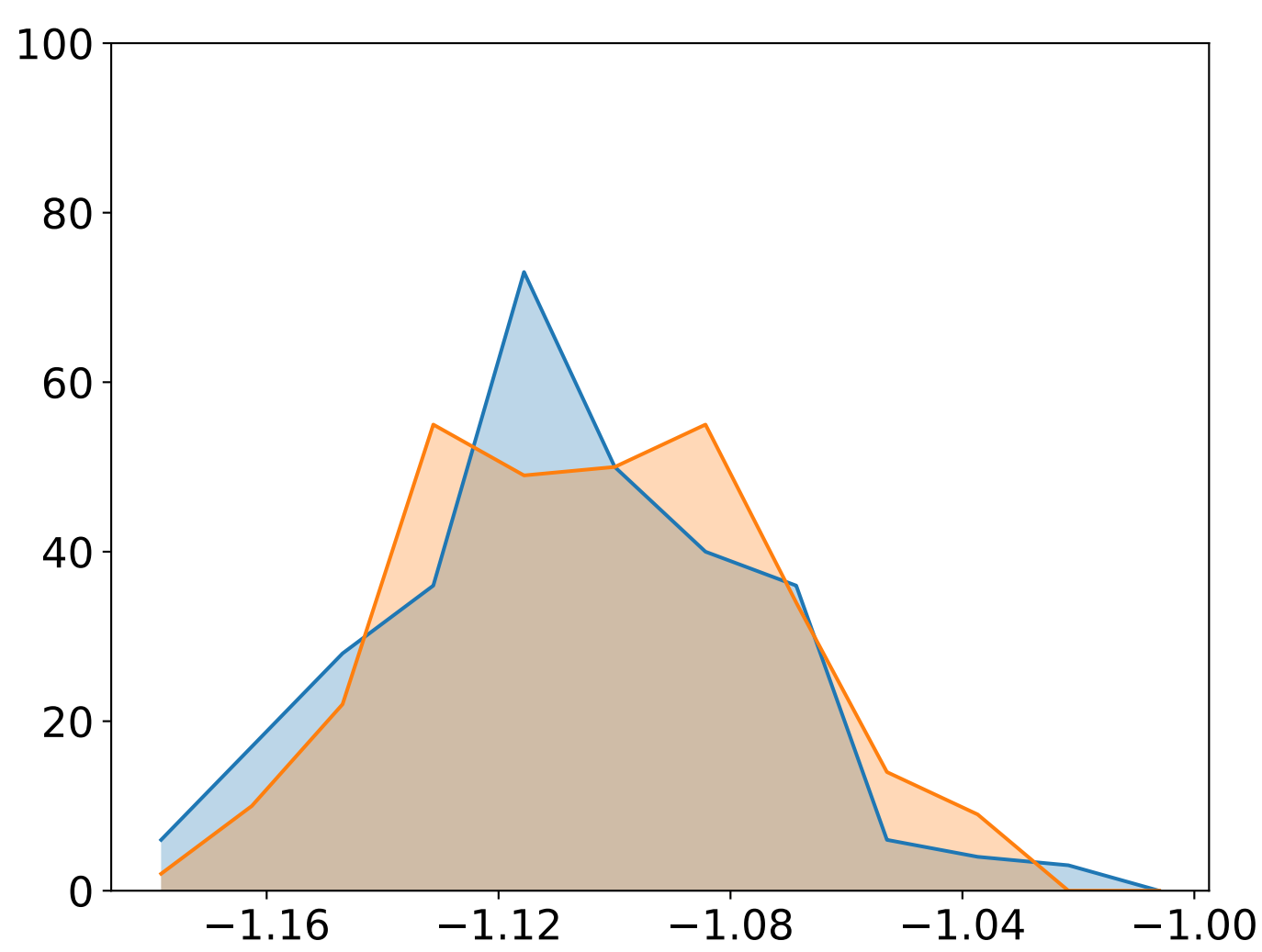
(b) J(x_m^*)
