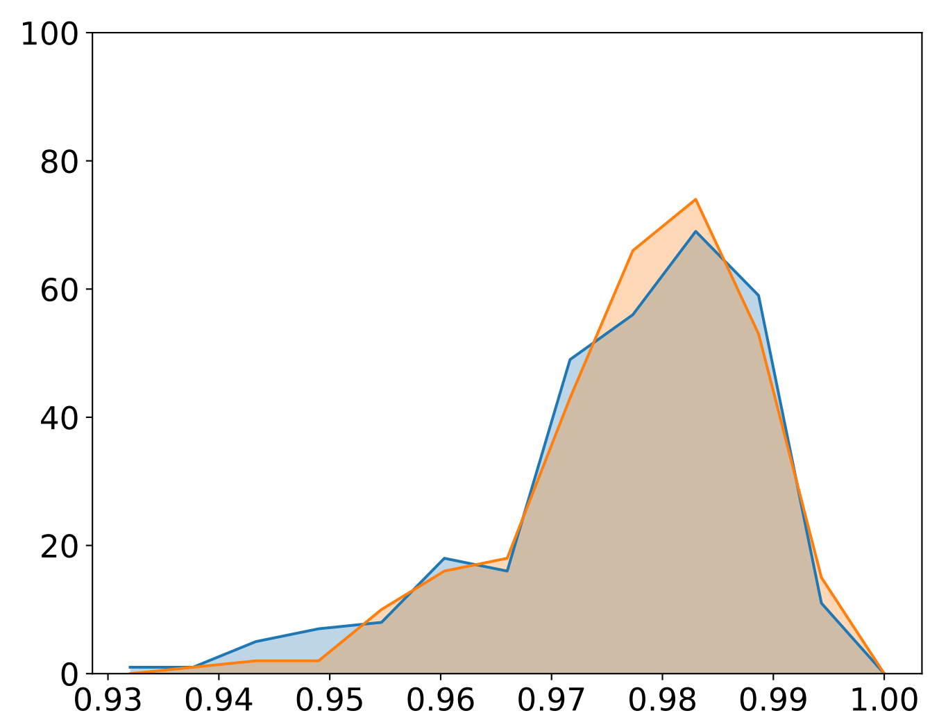
(c) CEC_{c,l}
