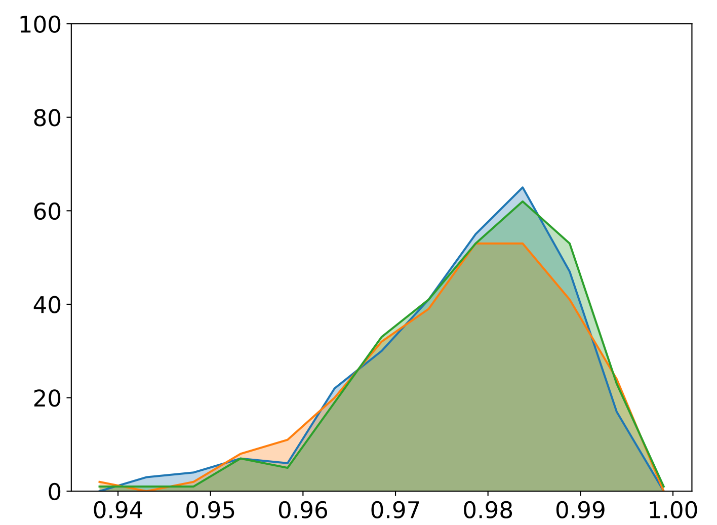
(c) CEC_{c,l}
