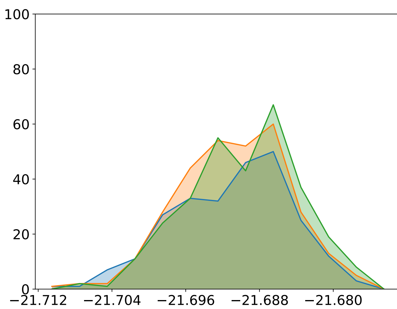
(b) J(x_m^*)
