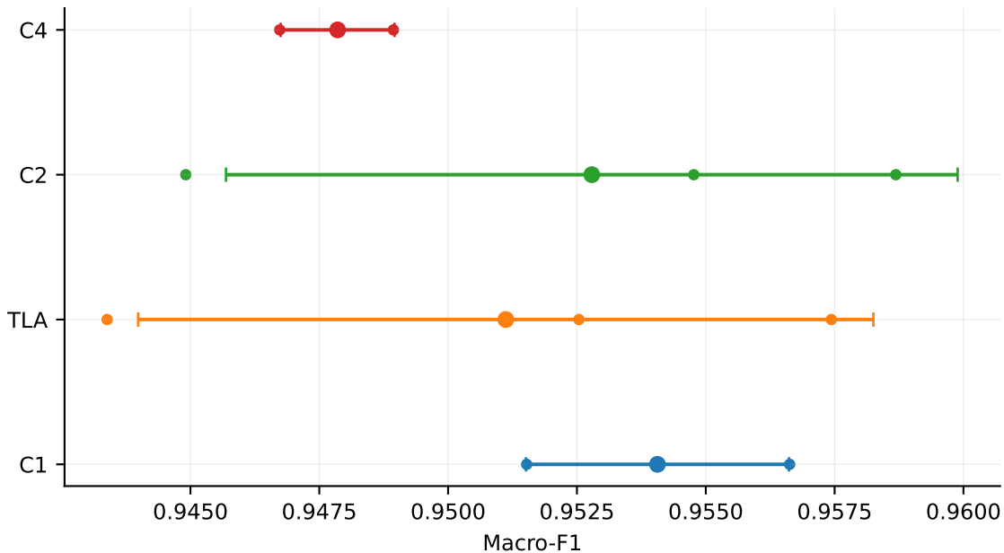
Token family: test Macro-F1 (mean \pm sd)
