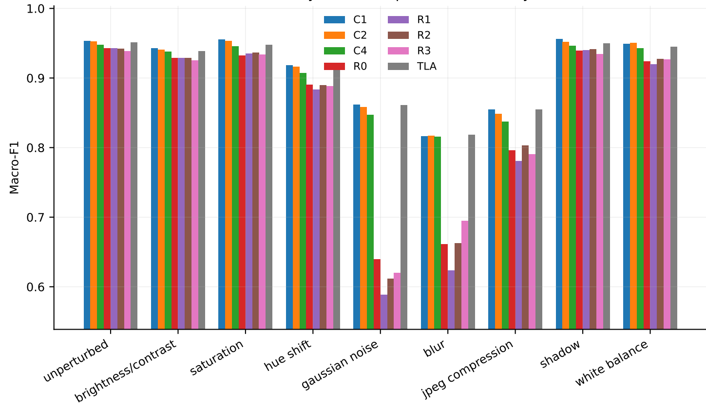
Macro-F1 by controlled perturbation family
