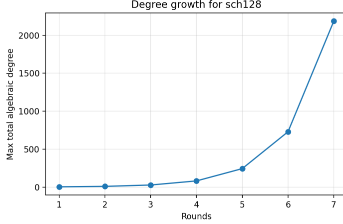
Figure 1: Algebraic degree growth of the composed permutation P as a function of composition depth k for the canonical SCH instantiation.
