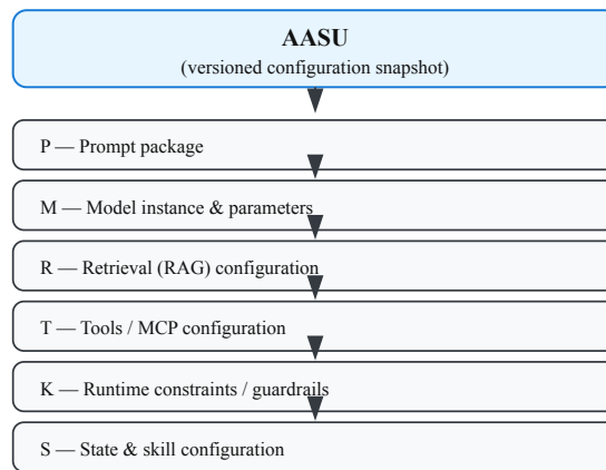
Figure 1. The Atomic AI Security Unit (AASU) as a configuration snapshot. Any change to P, M, R, T, K, S yields a distinct AASU that requires separate assurance.
