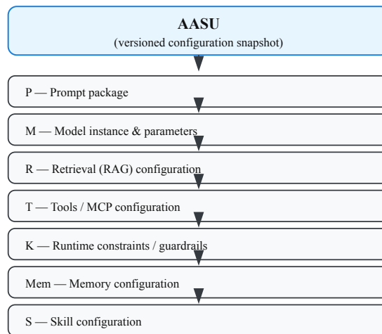
Figure 1. The Atomic AI Security Unit (AASU) as a configuration snapshot. Any change to P, M, R, T, K, Mem, S yields a distinct AASU that requires separate assurance.
