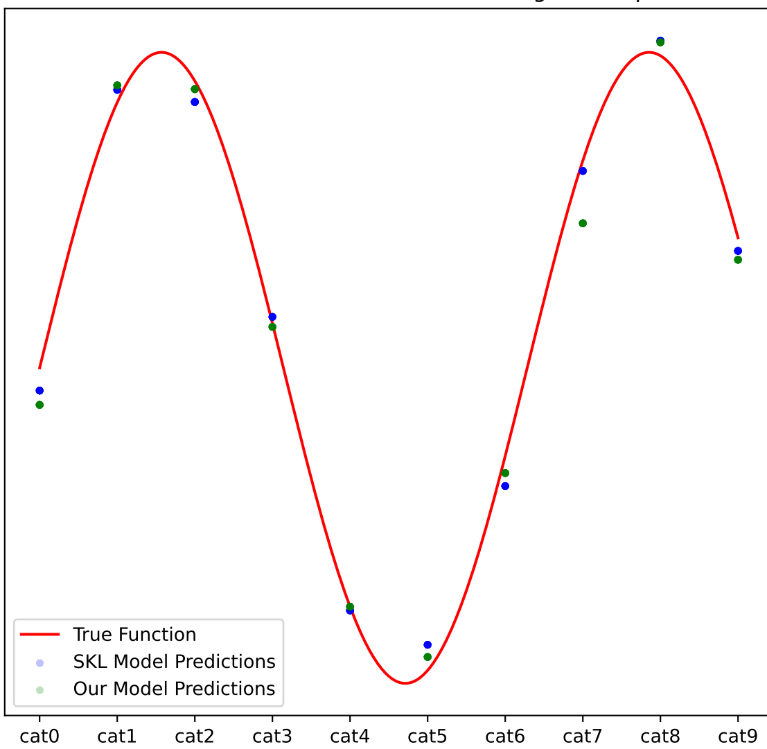
Feedforward Neural Network with categorical input
