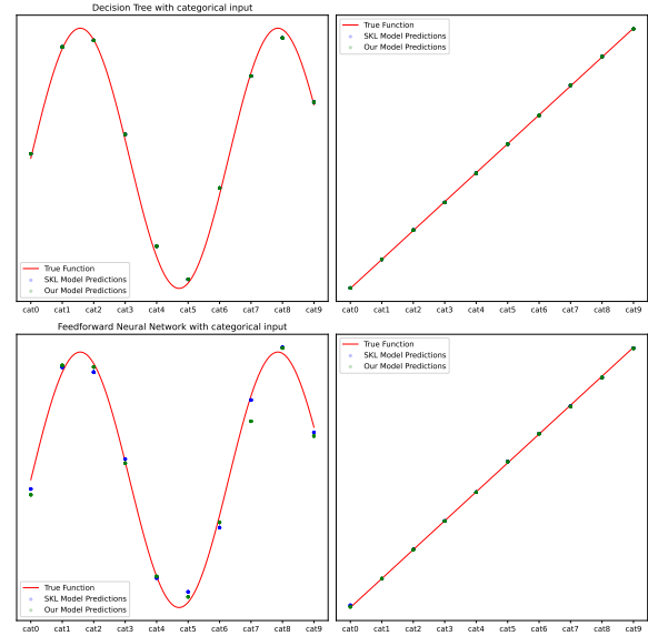
Figure 8: Comparison of our DT and FFNN implementations compared to the sklearn implementaion with categorical feature.
