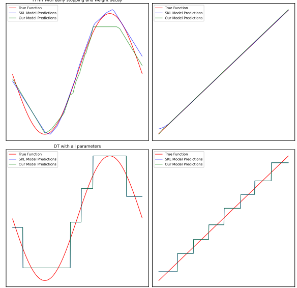
Figure 5: Example of comparison of our DT and FFNN implementations compared to the sklearn implementation with continuous feature.
