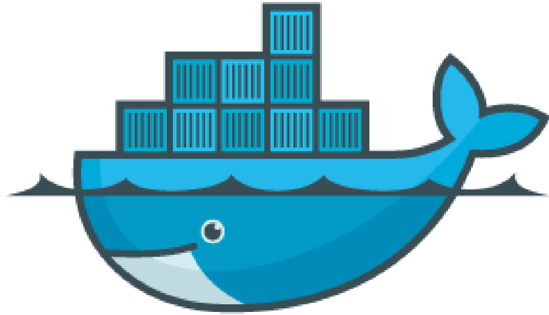
Docker – Containerization
