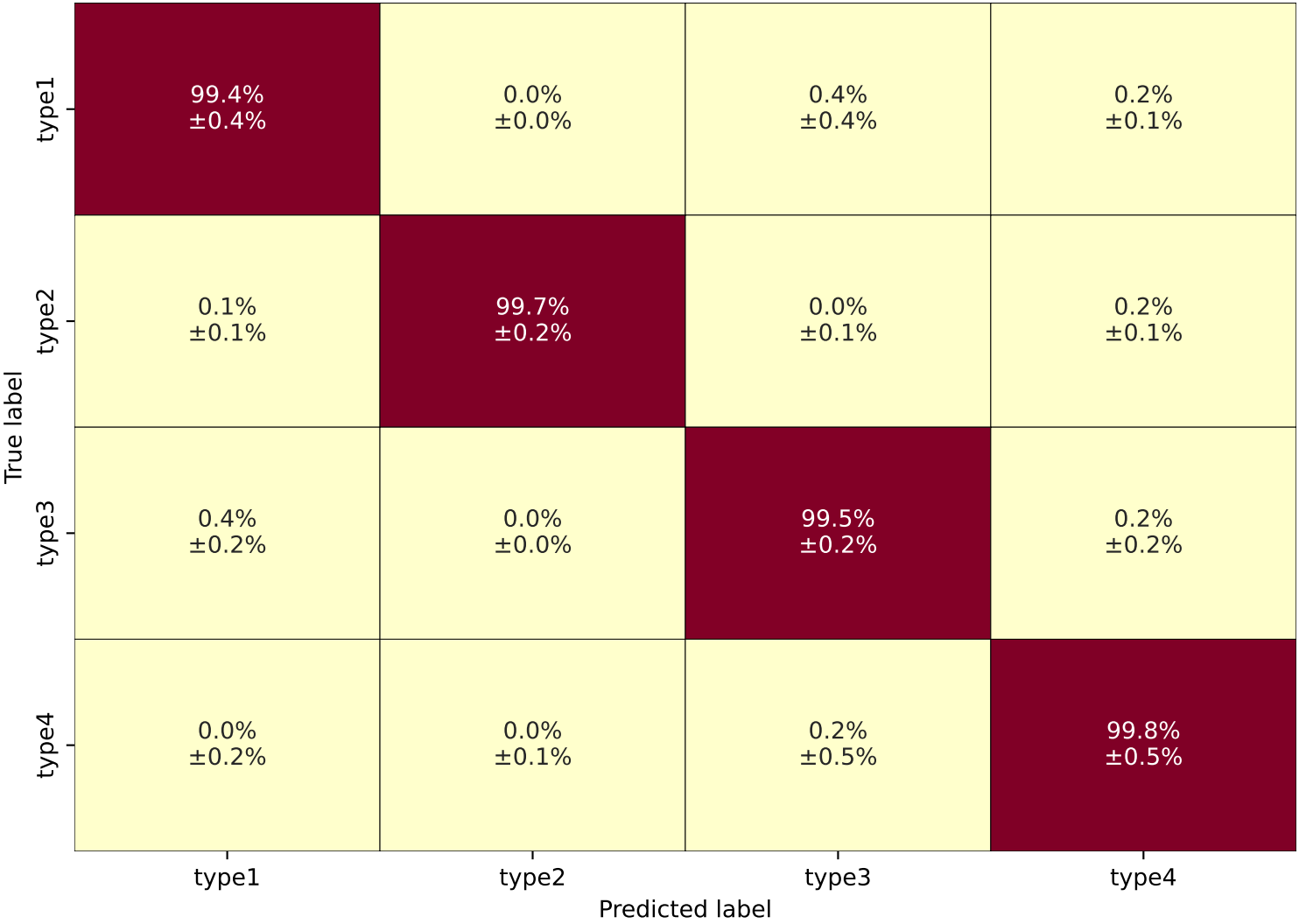
GREAC DENV Confusion Matrix
