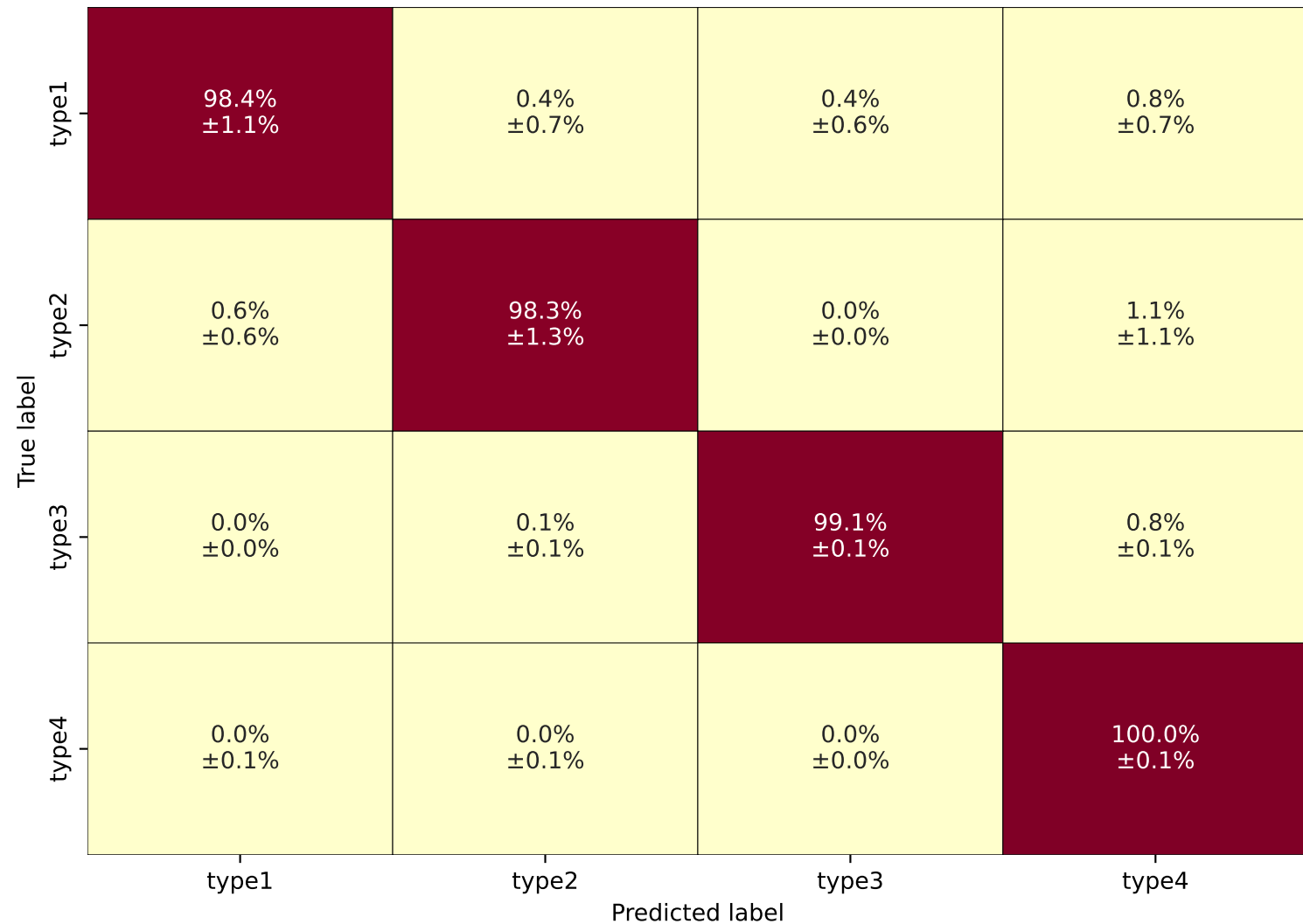
GREAC-Gaussian DENV Confusion Matrix
