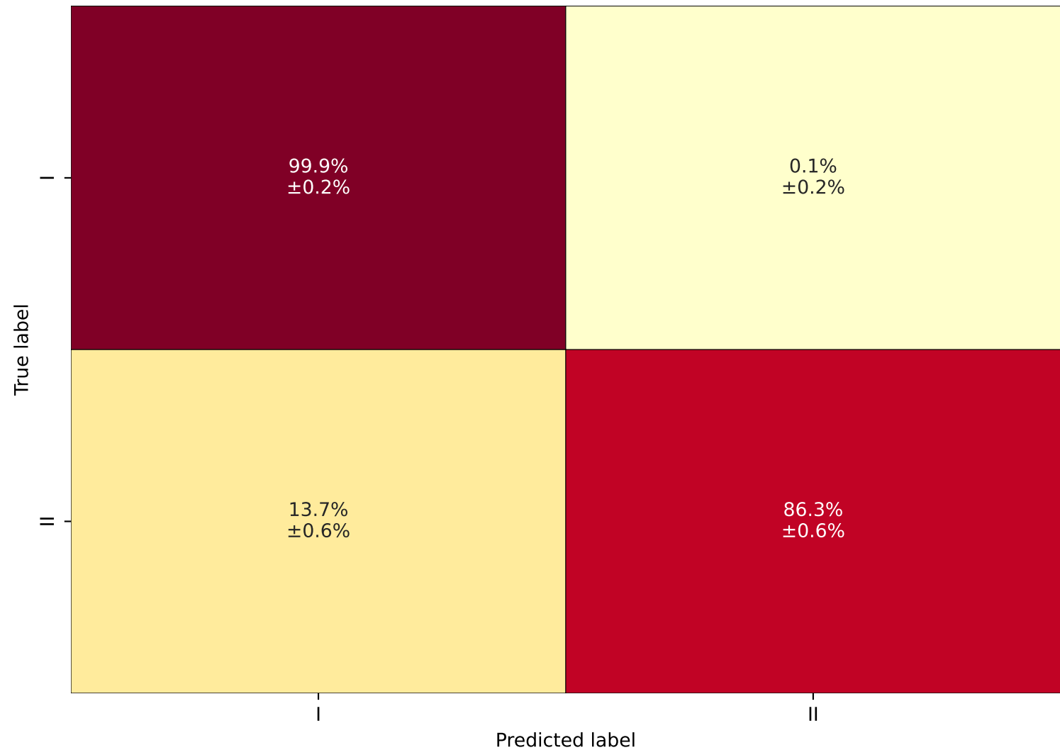
GREAC-Gaussian Monkeypox Confusion Matrix
