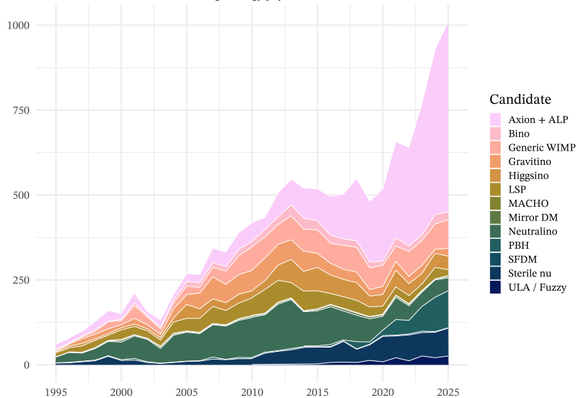
High-energy physics
