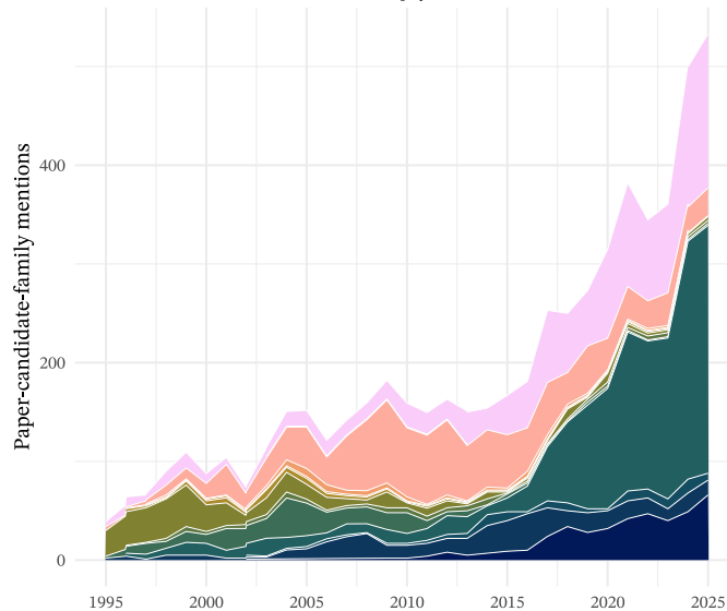
Astrophysics
