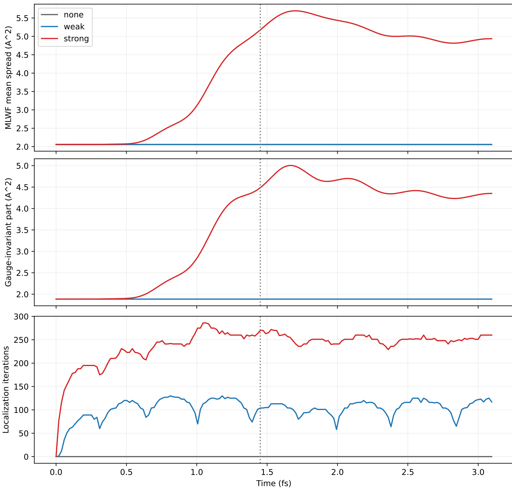
Si 4x4x4 k: MLWF updated every 10 RT steps Previous U reused; alpha feedback unchanged
