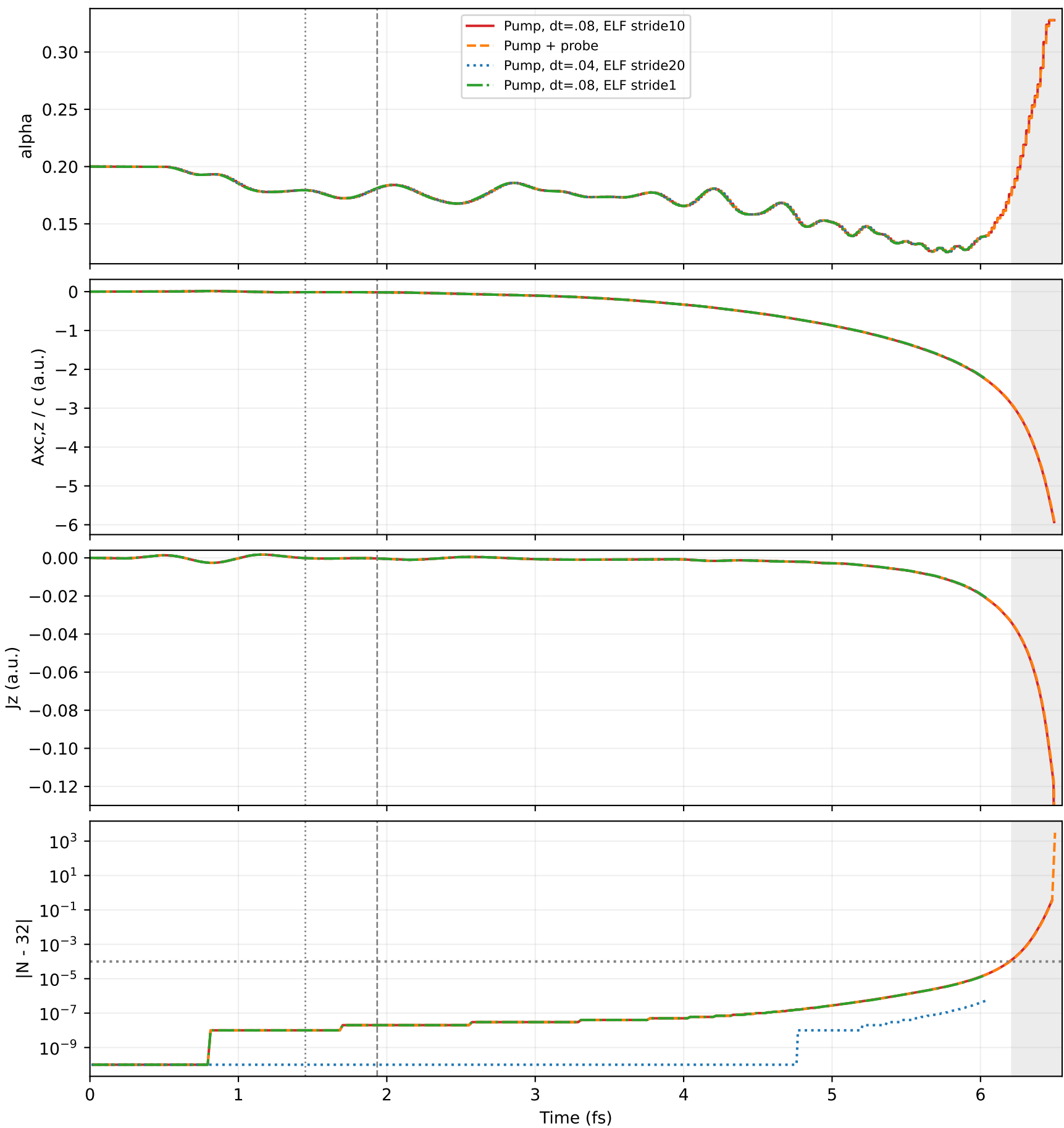
Si 4x4x4 k: strong pump cannot reach the spectral observation window Shading: electron-count error > 1e-4; late alpha is not physically reliable
