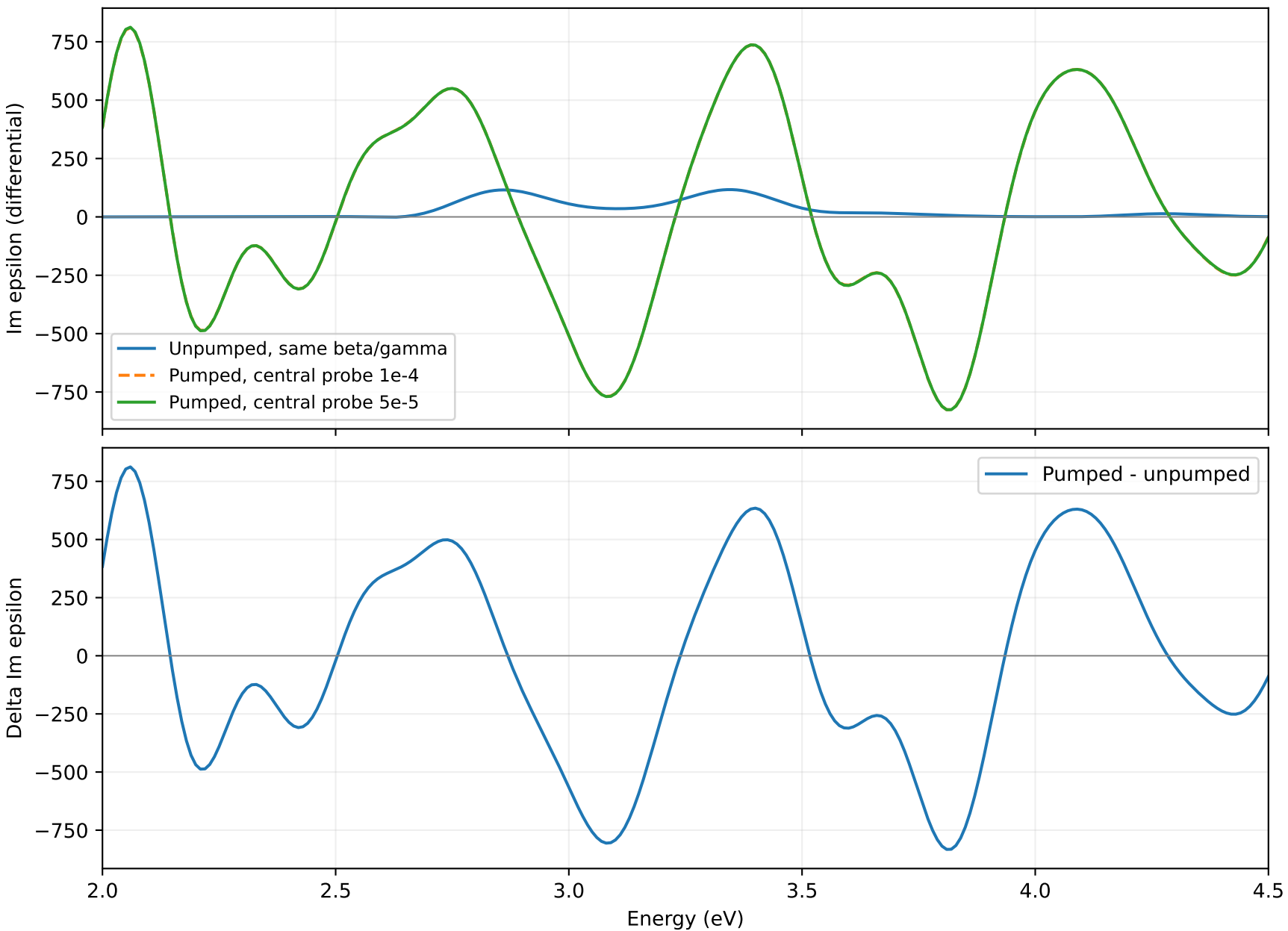
Si 4x4x4 k: dynamic ELF alpha + Proca, beta=0, gamma=0.001 Probe at 1.935 fs; 21.286 fs observation; pump 1e13 W/cm2
