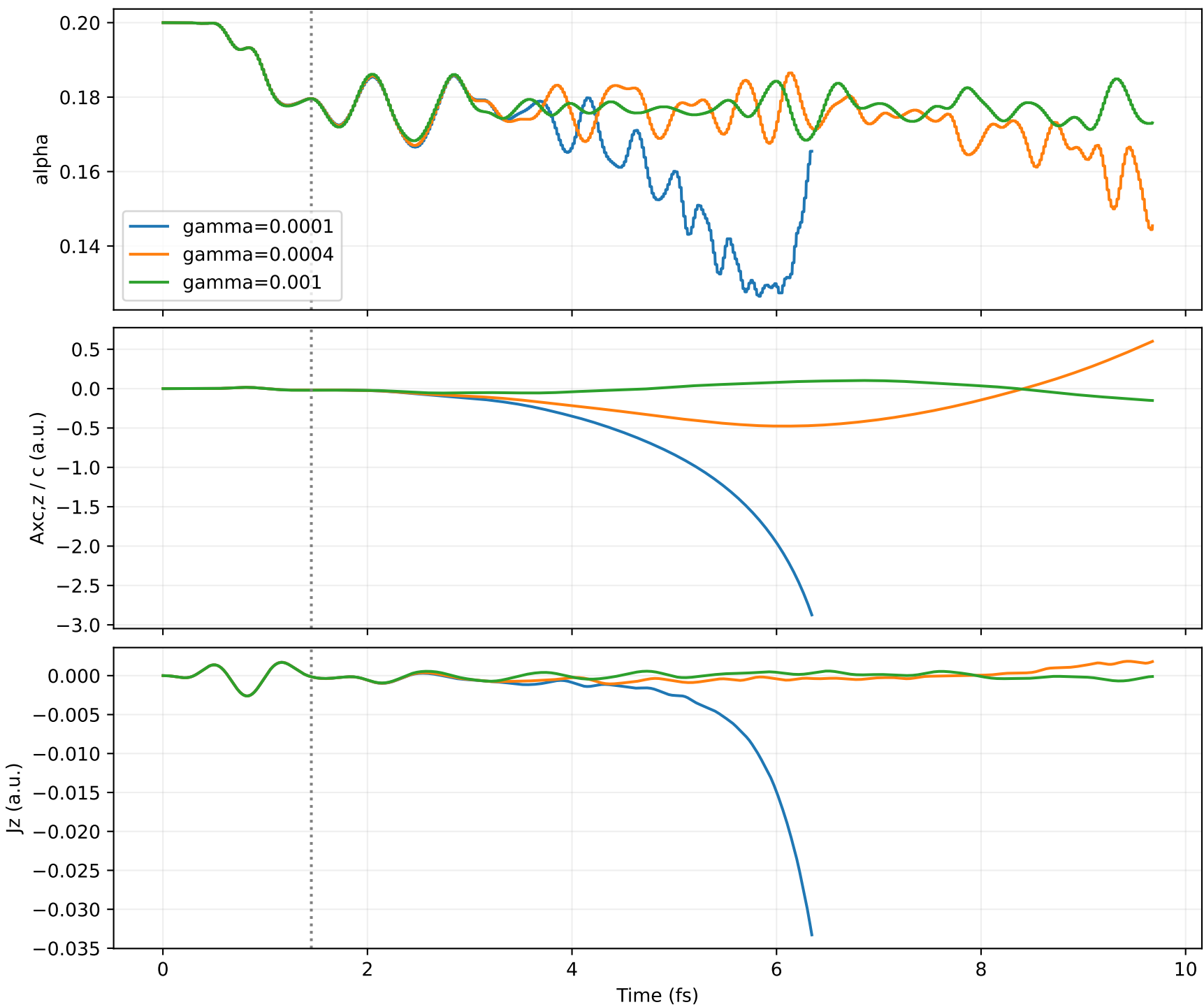
Si strong pump: ELF-Proca stability screen, beta=0 Gamma=1e-4 trace ends before norm error; other runs reach 9.68 fs
