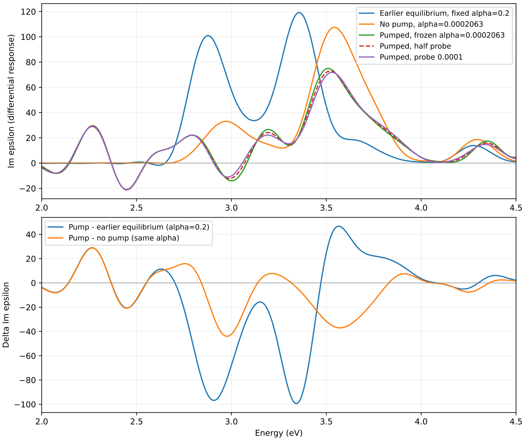
Si 4x4x4 k: frozen-screening pump-probe Probe at 1.935 fs, 21.286 fs observation, pump 1e13 W/cm2
