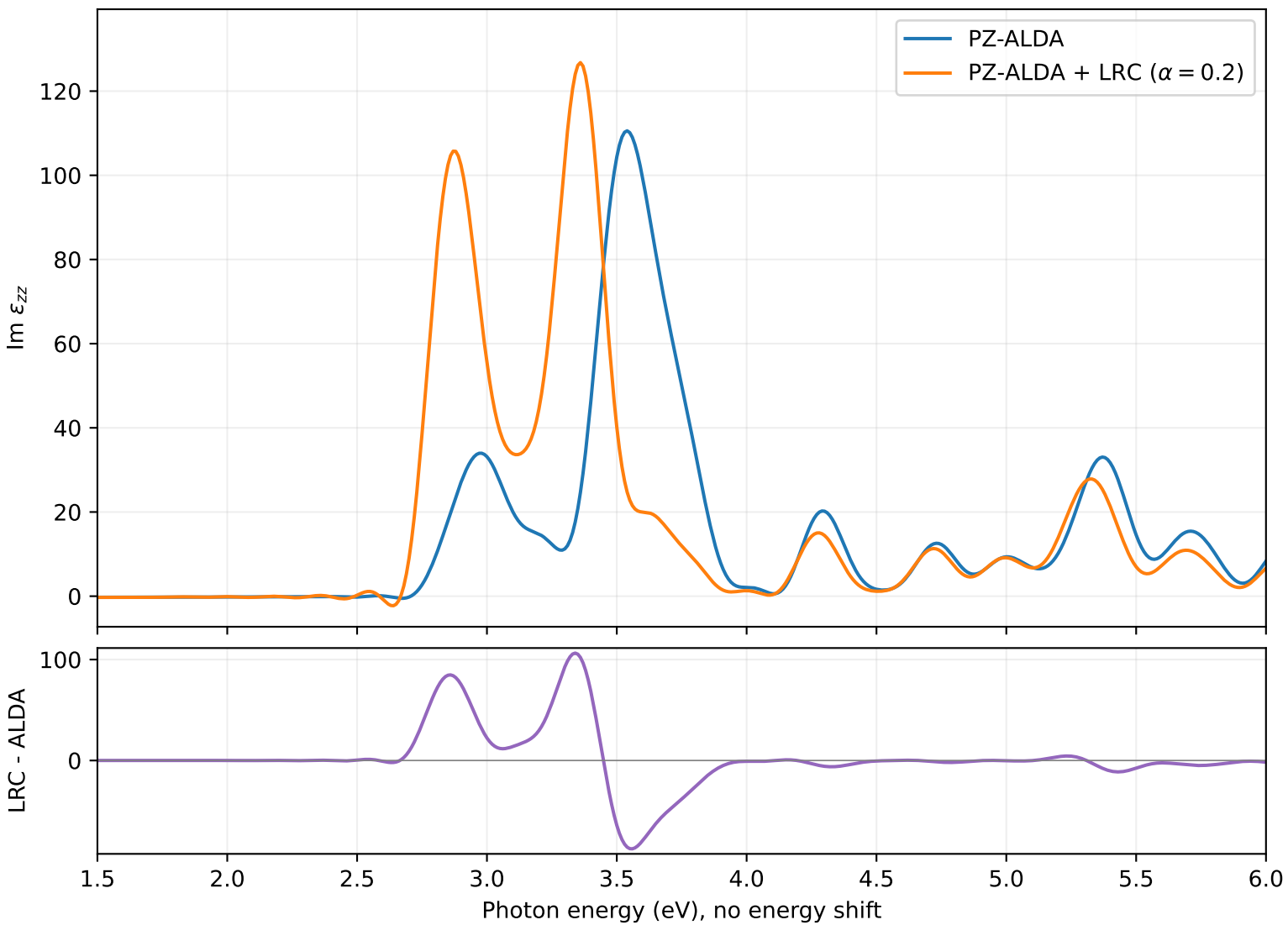
Si impulse response: fixed 4^3 k points
