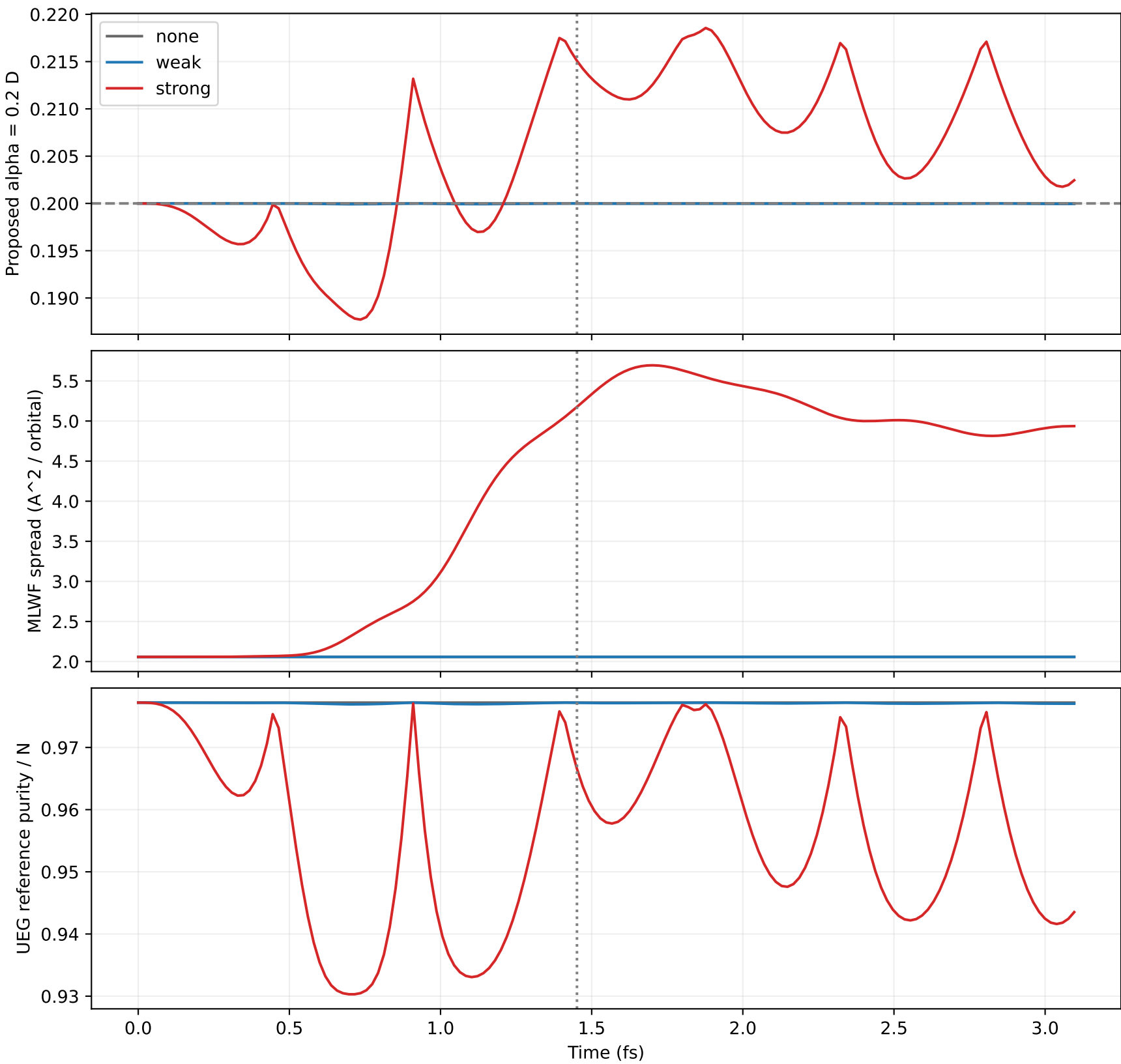
Si 4x4x4 k: UEG density-matrix distance Unclipped alpha; offline evaluation on previous trajectories
