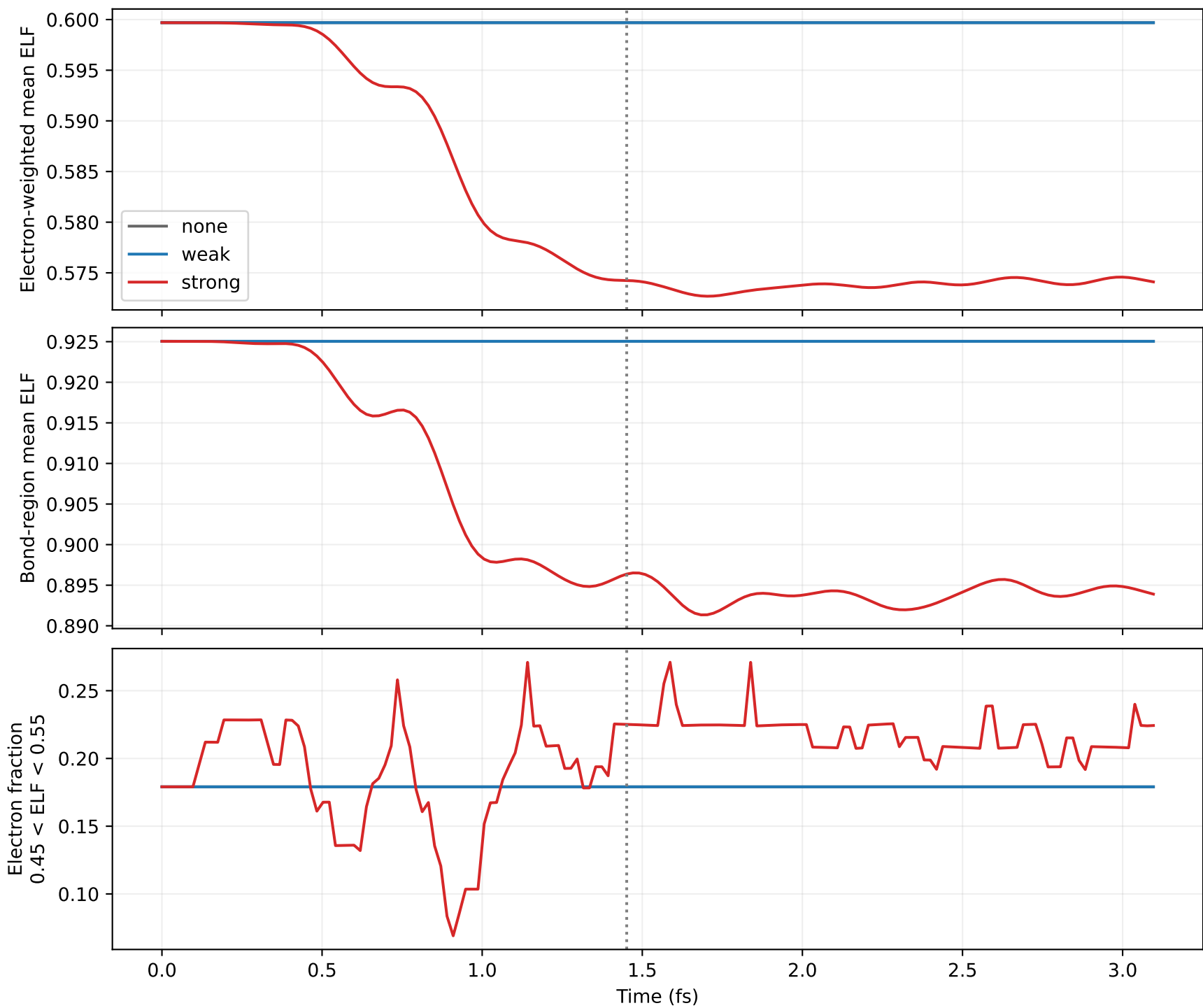
Si 4x4x4 k: current-corrected time-dependent ELF Existing trajectories; localization diagnostic, not a metallicity test
