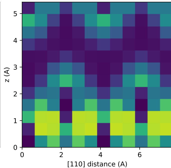
Strong: 3.096 fs
