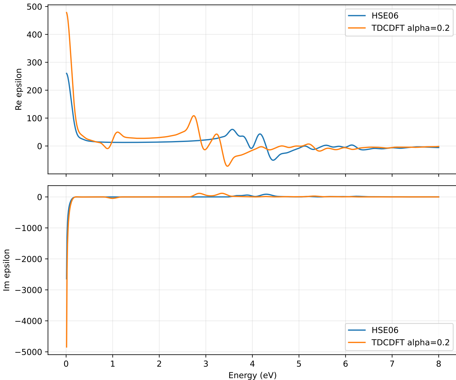
Si impulse: HSE06 vs fixed-alpha TDCDFT (21.29 fs)
