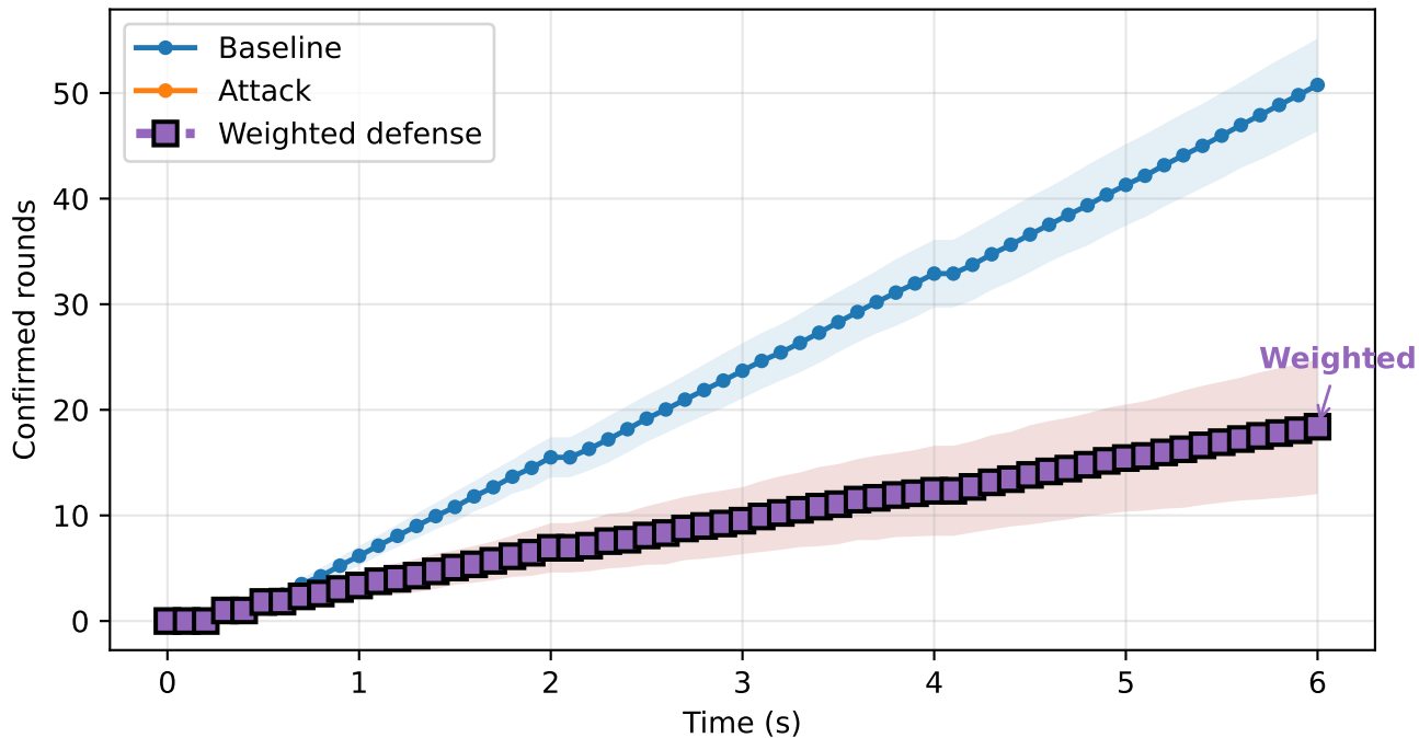
Weighted-defense comparison (30-seed mean \pm std)
