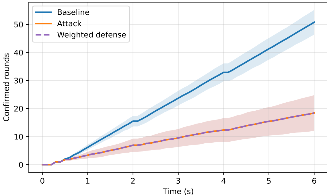
Weighted-defense comparison (30-seed mean \pm std)
