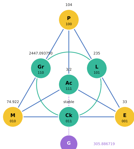
33 As • Arsenic
