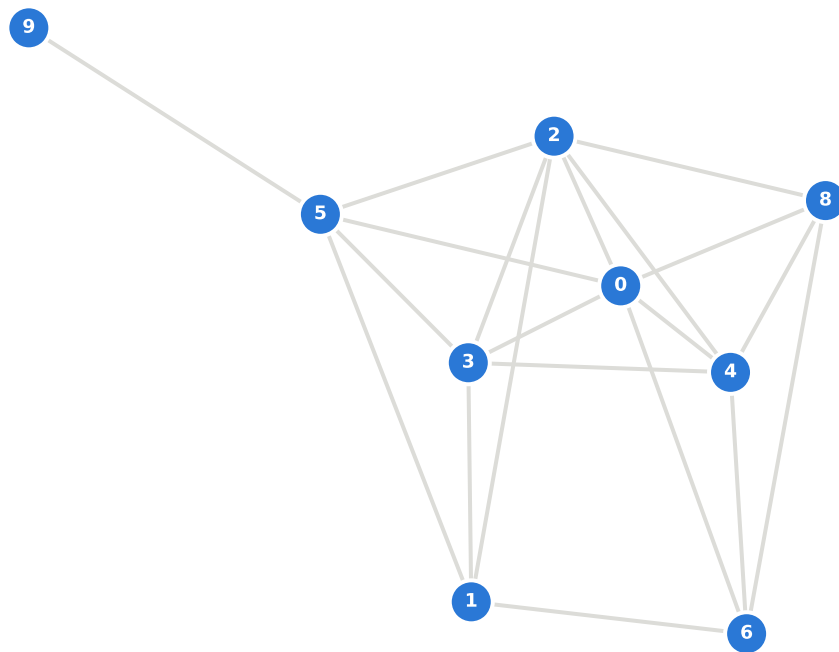
Abstract MHT incompatibility graph
