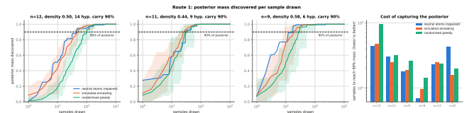
Figure 4: Posterior mass discovered against samples drawn.
