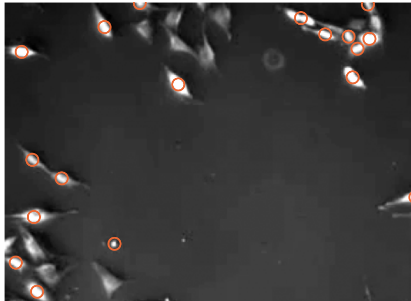
detections (crop)
