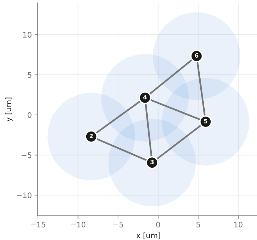
Optical-tweezer register (blockade half-discs)
