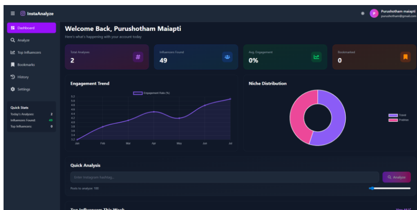
Figure 4: Dashboard Overview
