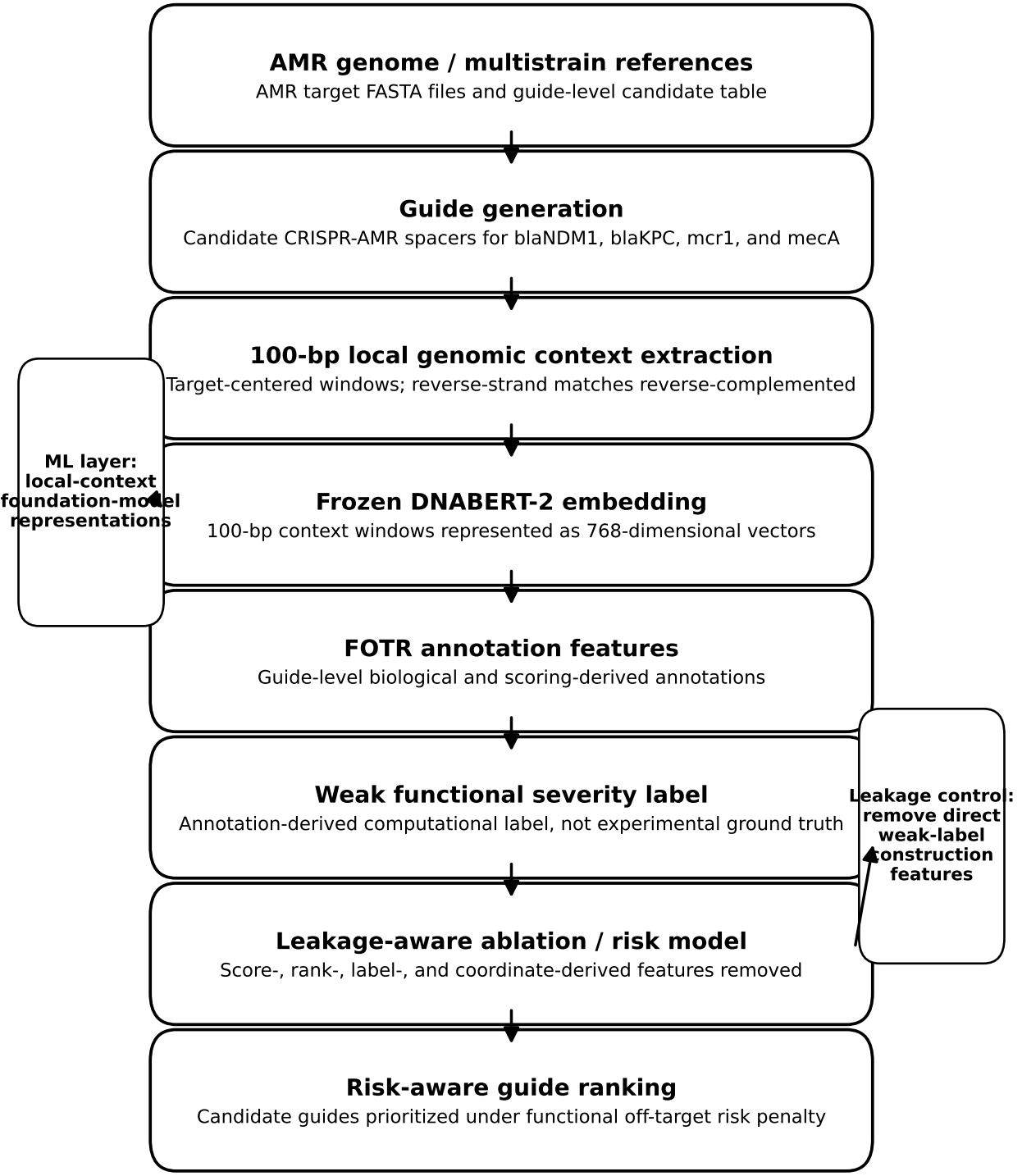
Figure 1. Context-aware FOTR-CRISPR + DNABERT-2 workflow
