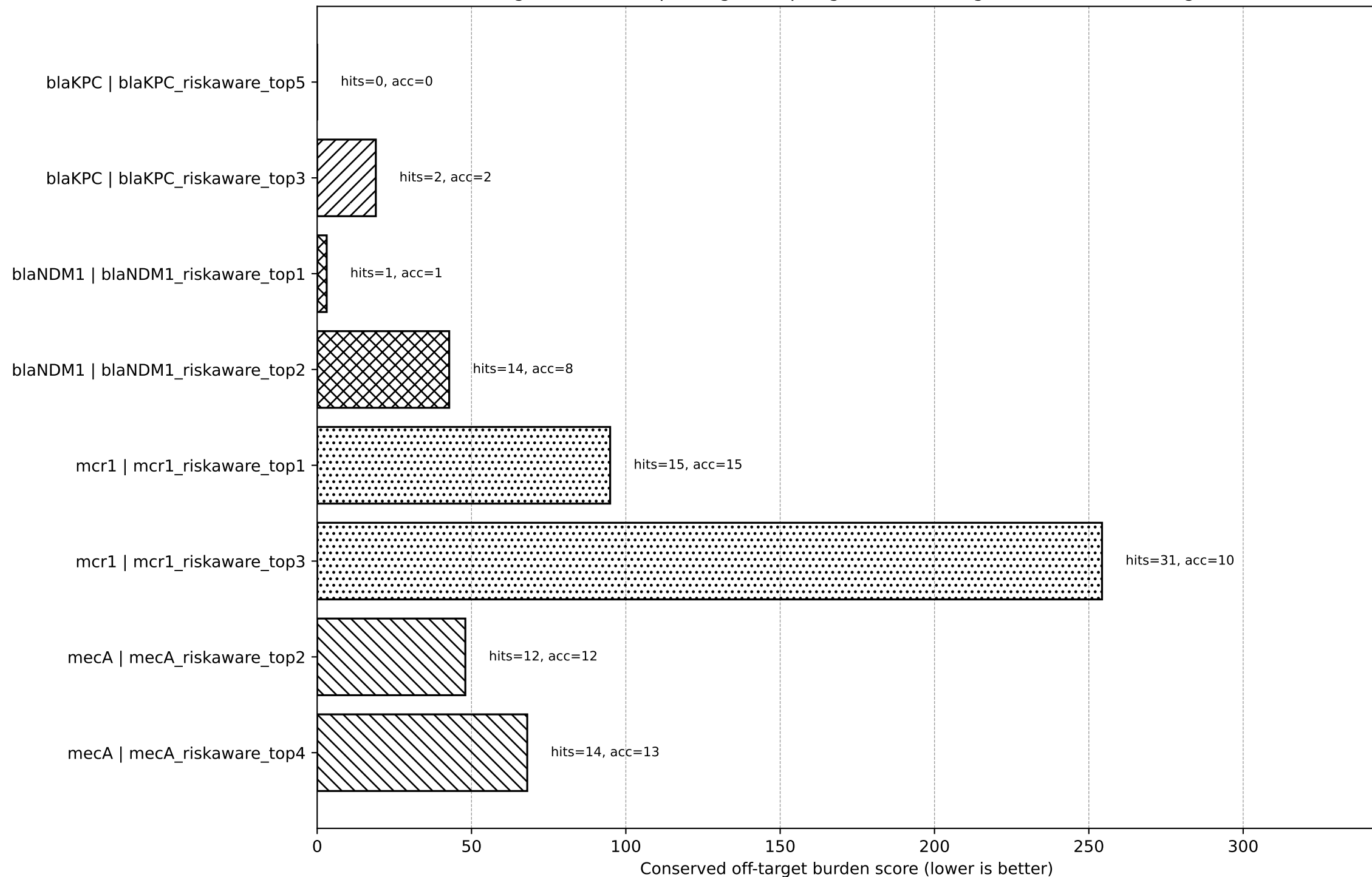
Figure 1. Final top two guides per gene after integrated FOTR screening
