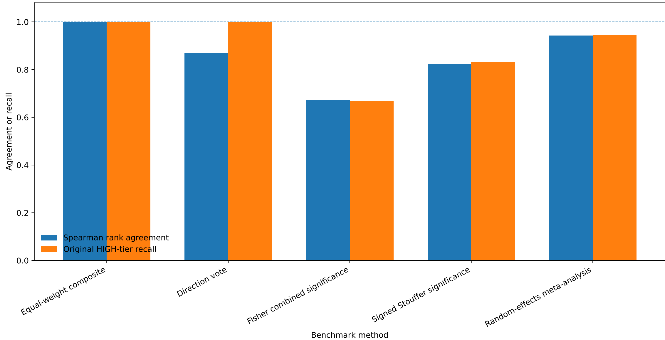
MCI agreement with simpler benchmark methods
