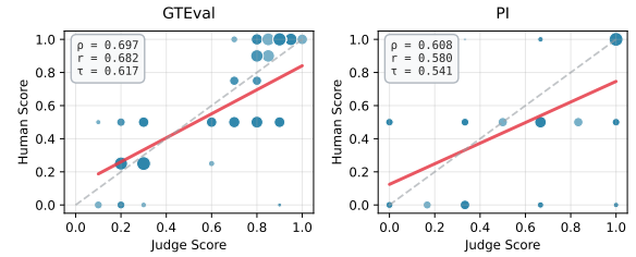
Figure 4: Judge-human correlation on ChatbotArena: Correlation of Claude-4-Sonnet judge scores & human scores for GTEval and PI, evaluated on Gemini-2.5-Pro user-proxy outputs ( N=100 per metric). Solid line: linear fit; dashed: identity. Point size encodes local sample density. All correlations p < 0.001 .
