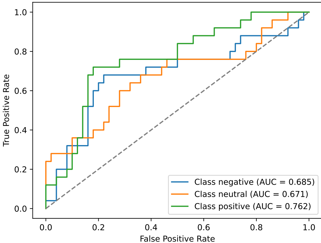
ROC Curve (One-vs-Rest)
