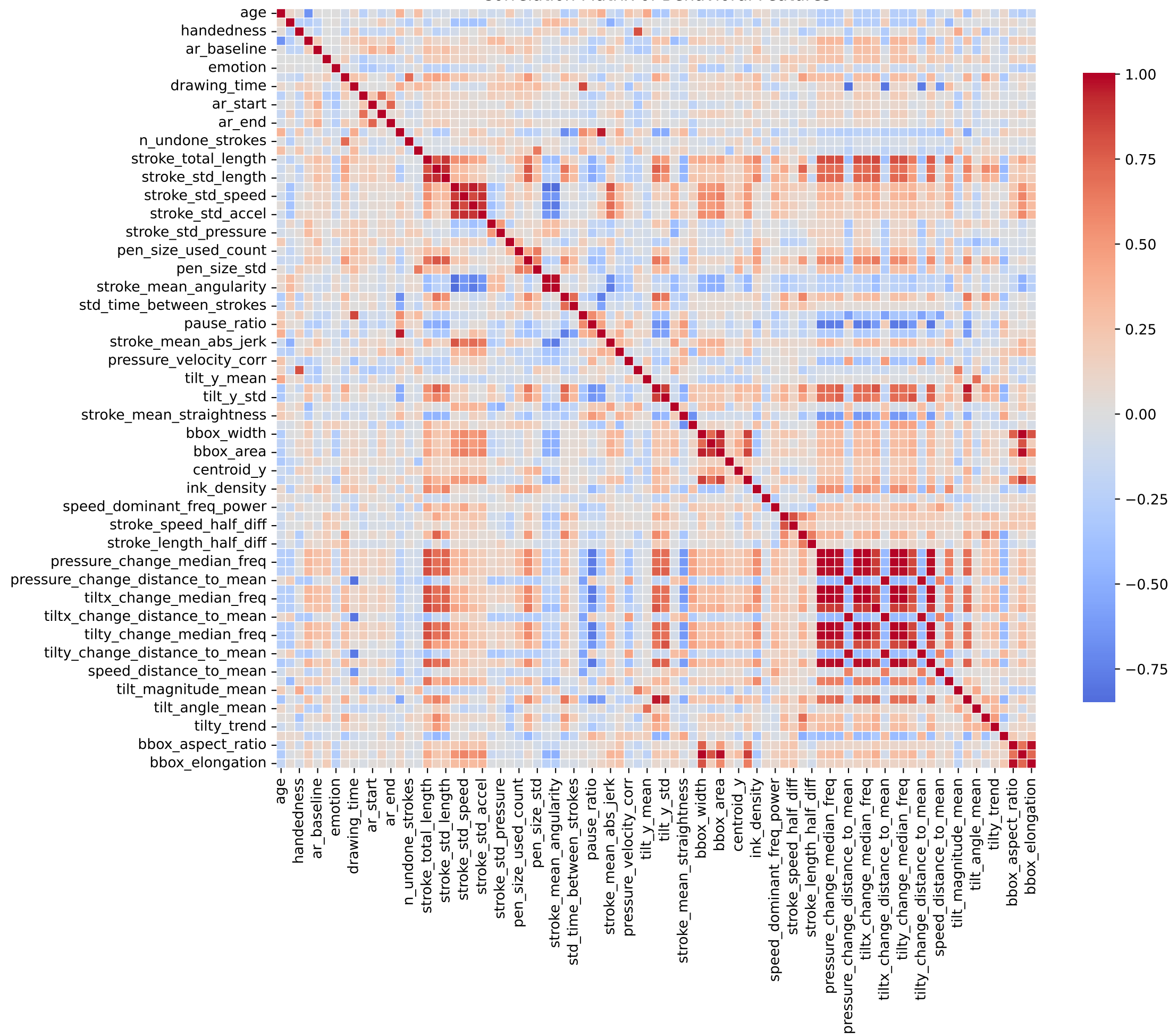
Correlation Matrix of Behavioral Features
