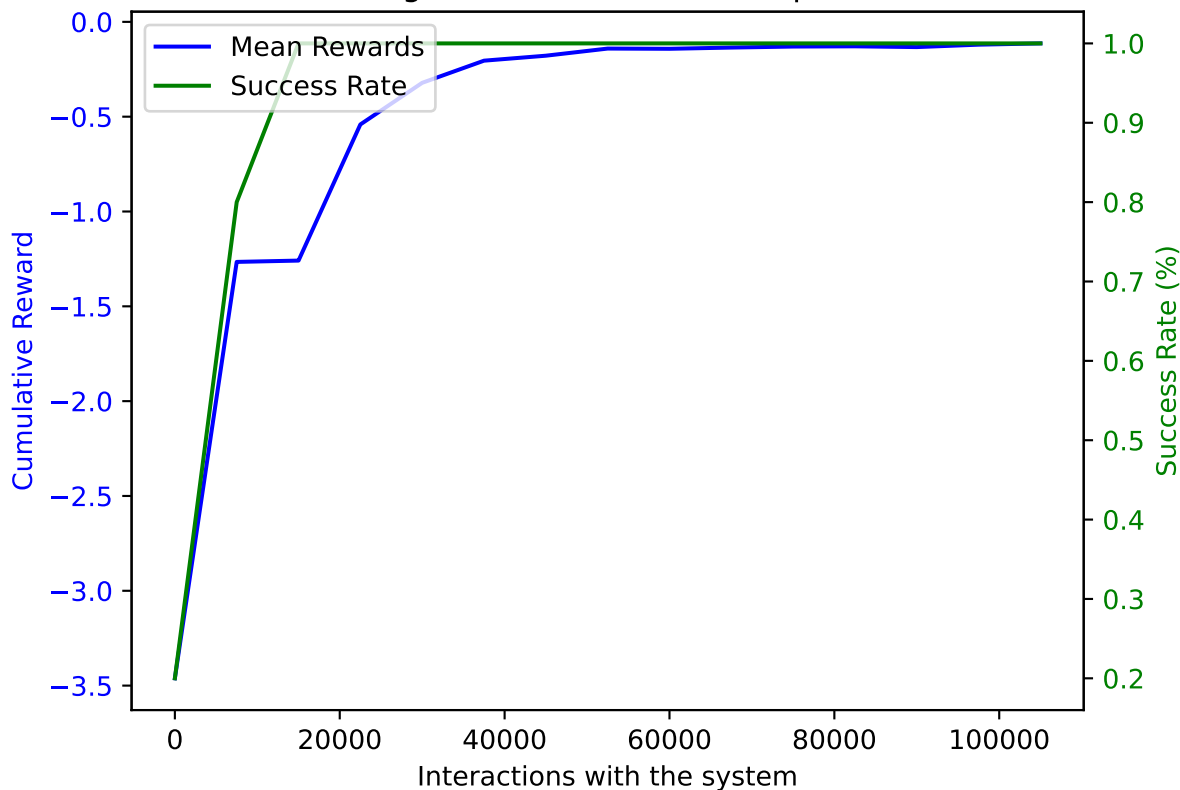
PPO on AWAKE with DoF: 1 and trained on 105000 samples averaged over 10 validation episodes
