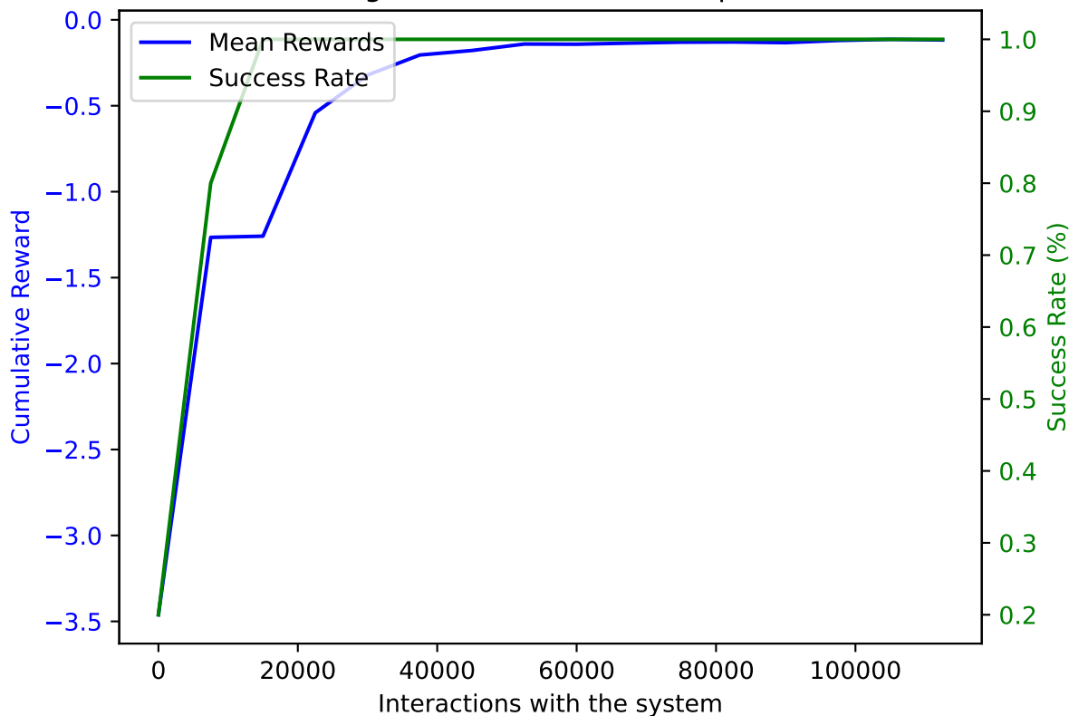
PPO on AWAKE with DoF: 1 and trained on 112500 samples averaged over 10 validation episodes
