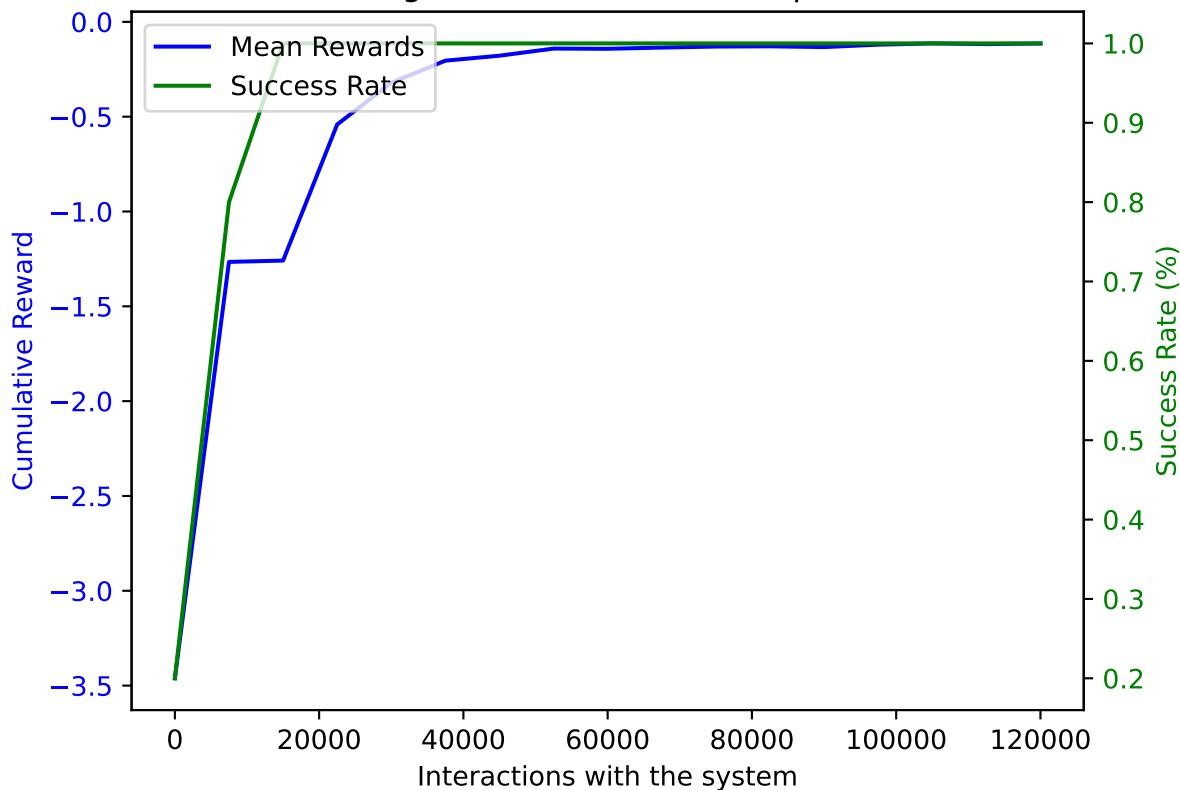
PPO on AWAKE with DoF: 1 and trained on 120000 samples averaged over 10 validation episodes
