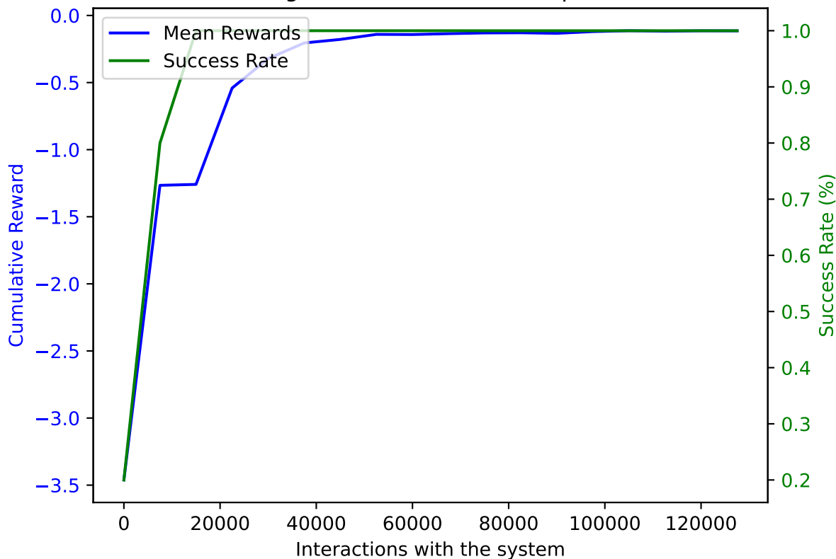
PPO on AWAKE with DoF: 1 and trained on 127500 samples averaged over 10 validation episodes
