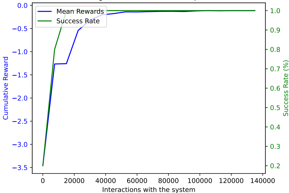
PPO on AWAKE with DoF: 1 and trained on 135000 samples averaged over 10 validation episodes
