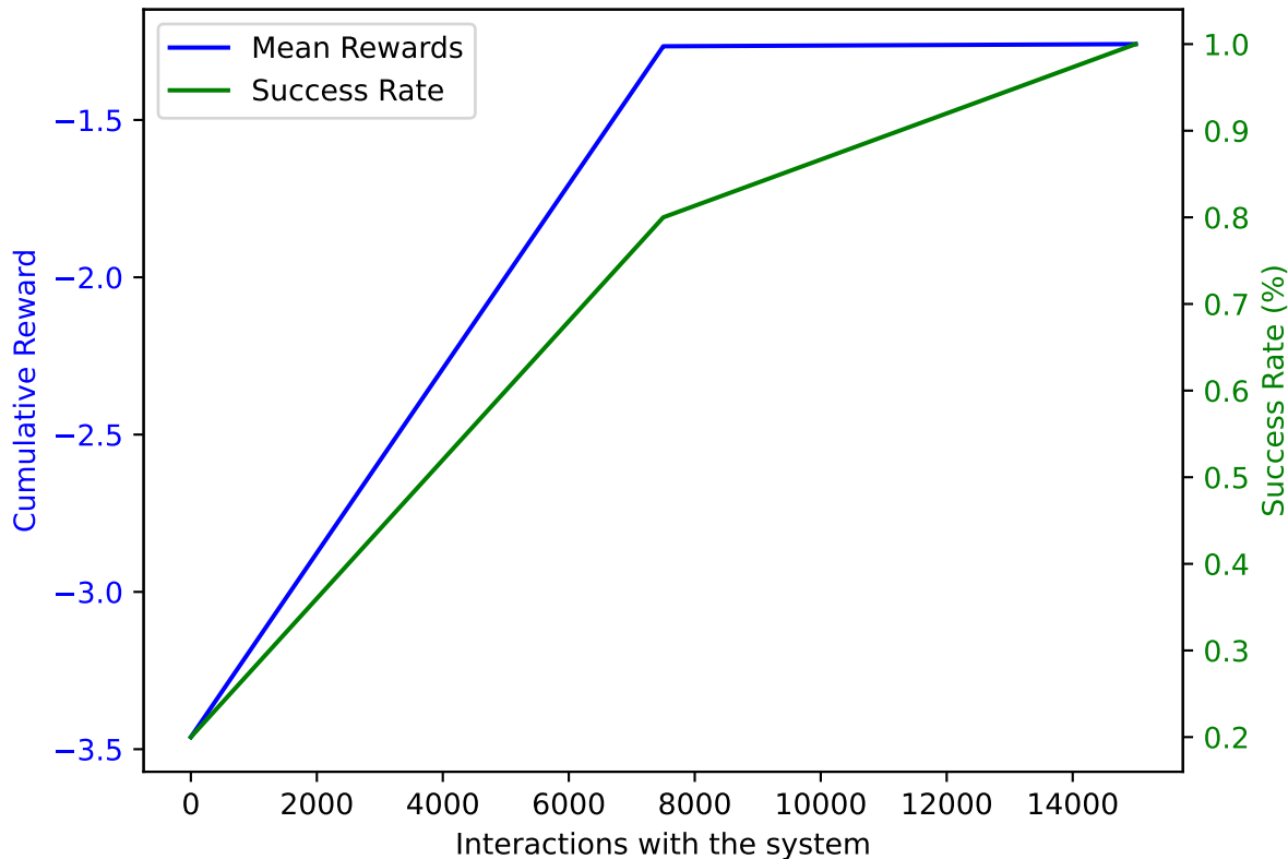
PPO on AWAKE with DoF: 1 and trained on 15000 samples averaged over 10 validation episodes
