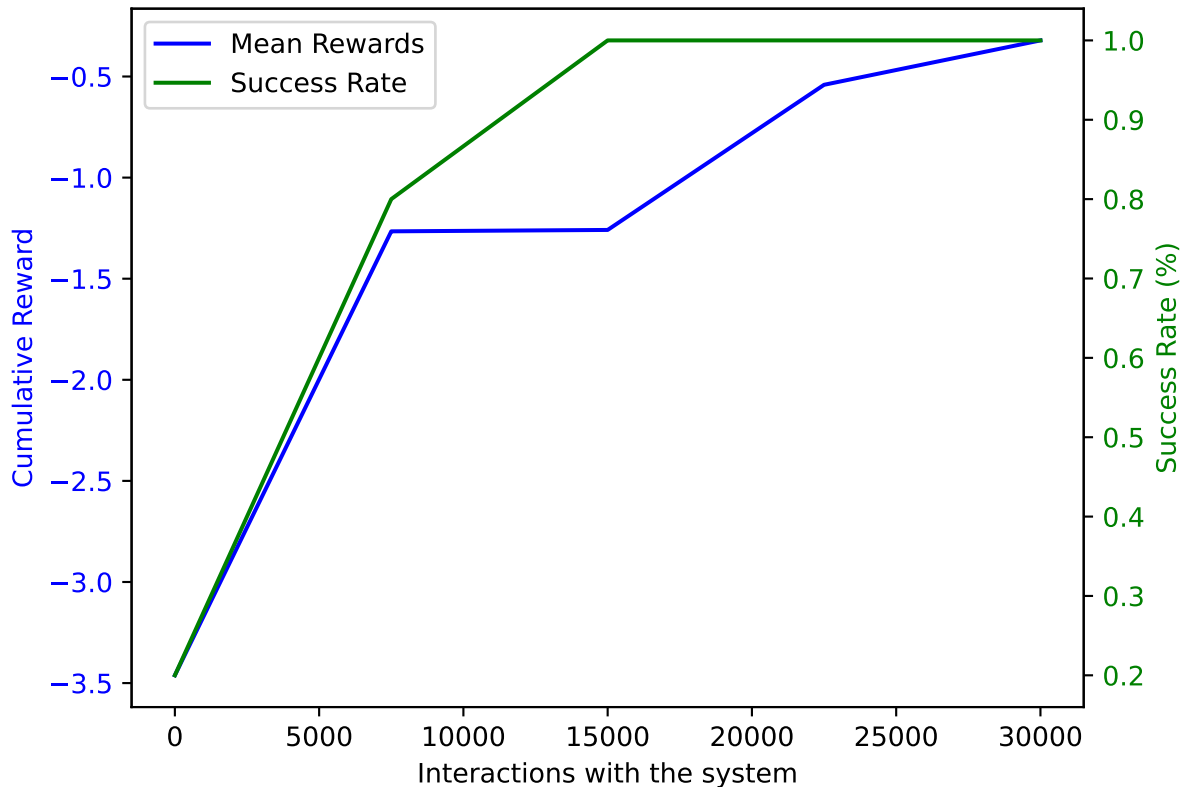
PPO on AWAKE with DoF: 1 and trained on 30000 samples averaged over 10 validation episodes
